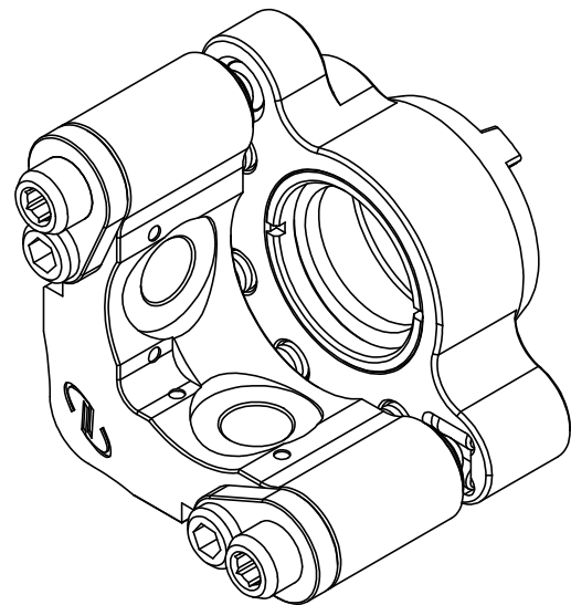
MODEL ST50T-R2H REAR LOAD, 2 HEX ADJUSTORS
